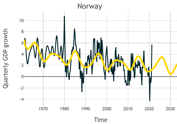
Figure 19: harmonic regression fit for Norway.
