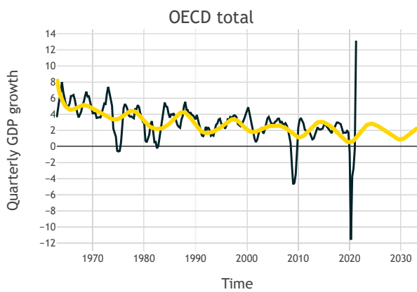
Figure 21: harmonic regression fit for all OECD countries.
