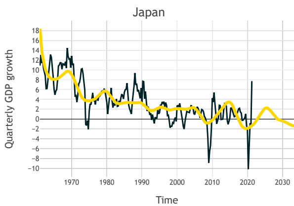
Figure 15: harmonic regression fit for Japan.
