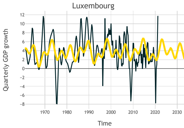
Figure 17: harmonic regression fit for Luxembourg.
