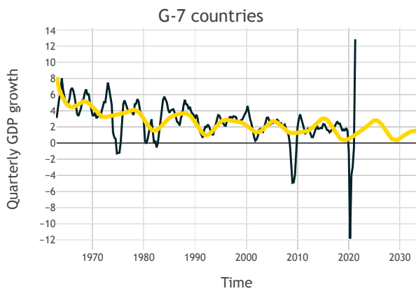
Figure 9: harmonic regression fit for G-7 countries.
