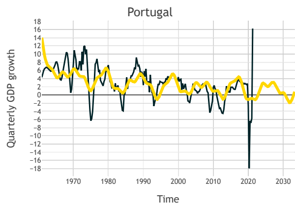
Figure 22: harmonic regression fit for Portugal.
