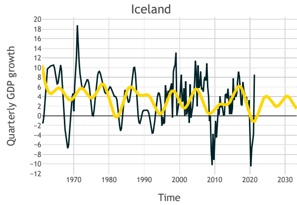
Figure 12: harmonic regression fit for Iceland.
