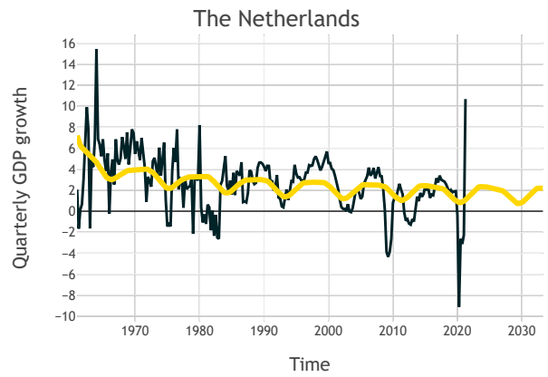
Figure 26: harmonic regression fit for The Netherlands.
