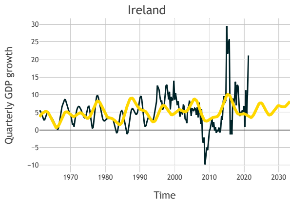
Figure 13: harmonic regression fit for Ireland.
