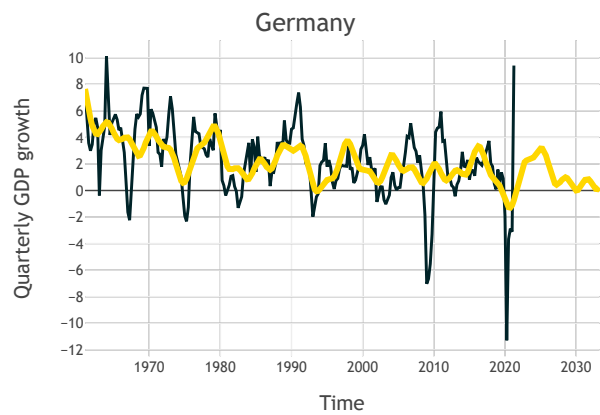
Figure 10: harmonic regression fit for Germany.
