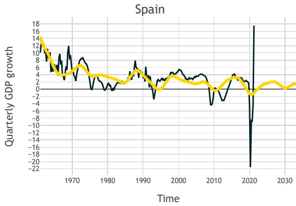
Figure 23: harmonic regression fit for Spain.
