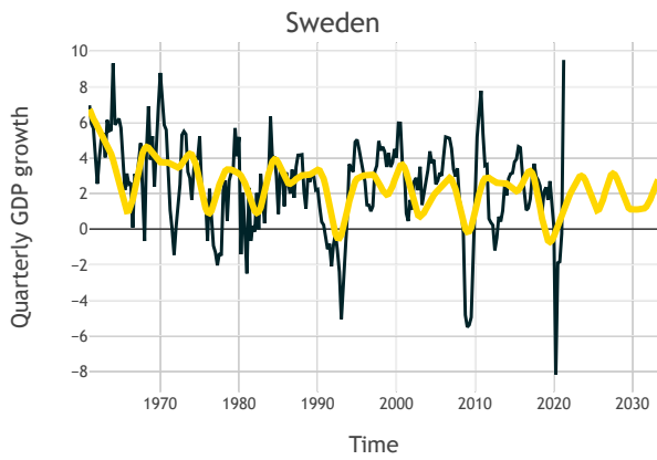
Figure 25: harmonic regression fit for Sweden.
