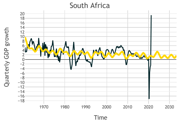
Figure 24: harmonic regression fit for South Africa.
