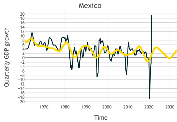
Figure 18: harmonic regression fit for Mexico.
