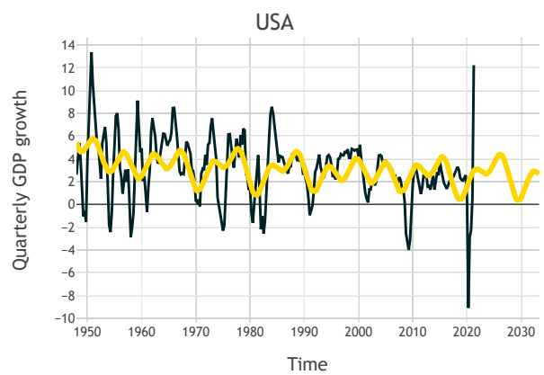
Figure 28: harmonic regression fit for USA.
