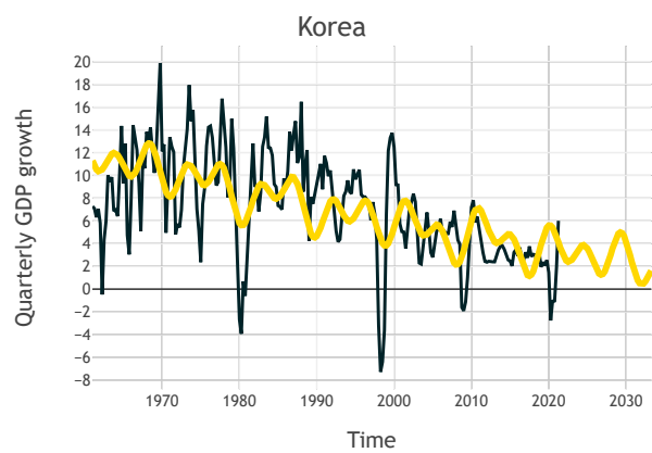
Figure 16: harmonic regression fit for Korea.
