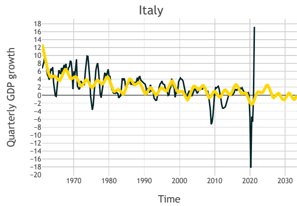
Figure 14: harmonic regression fit for Italy.
