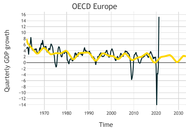
Figure 20: harmonic regression fit for the European OECD countries.
