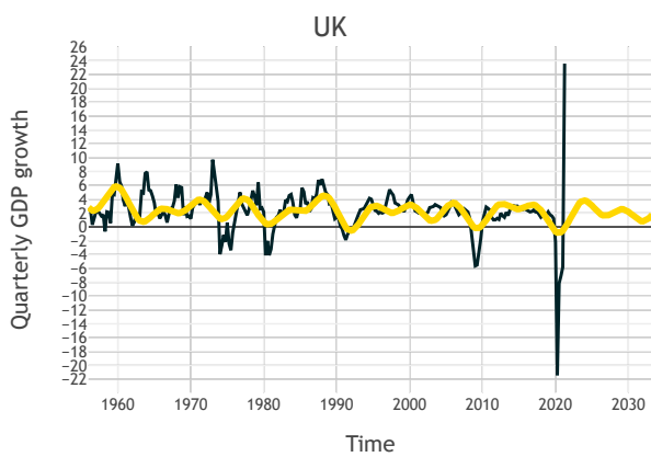
Figure 27: harmonic regression fit for UK.
